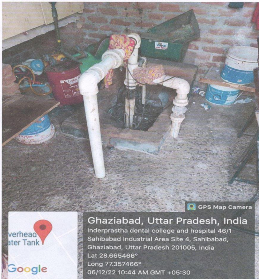
BOREWELL INSTALLATION
